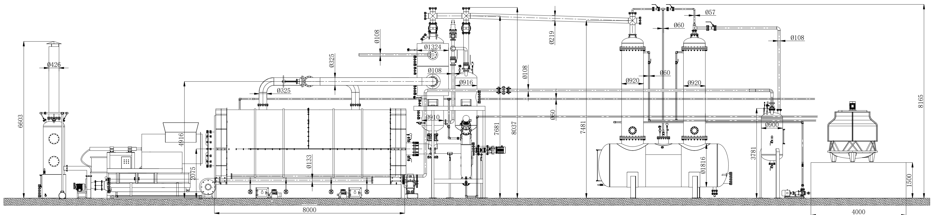
BLJ-16立面图(仅供参考) BLJ-16 Elevation (for reference only)
